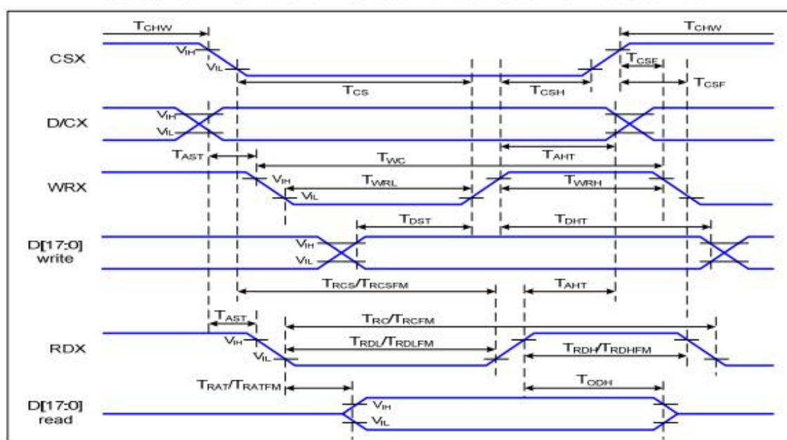
Figure 1 Parallel Interface Timing Characteristics (8080-Series MCU Interface)
