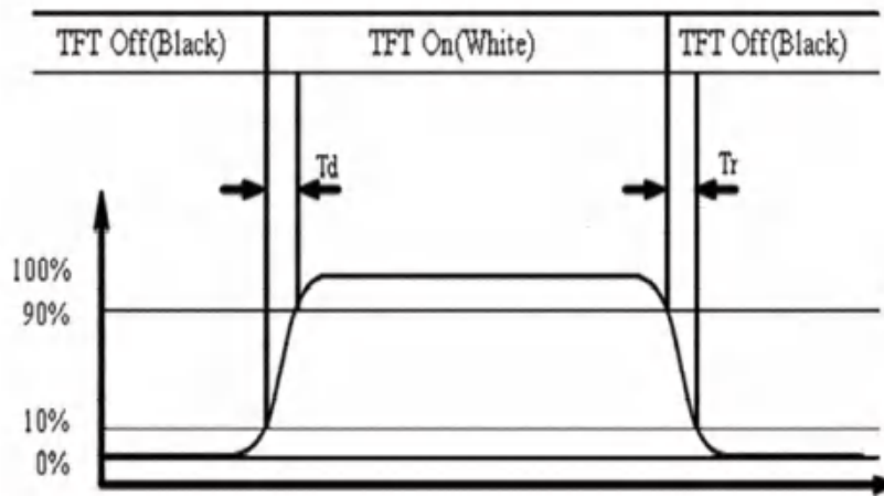
Figure 4. Response Time Testing
